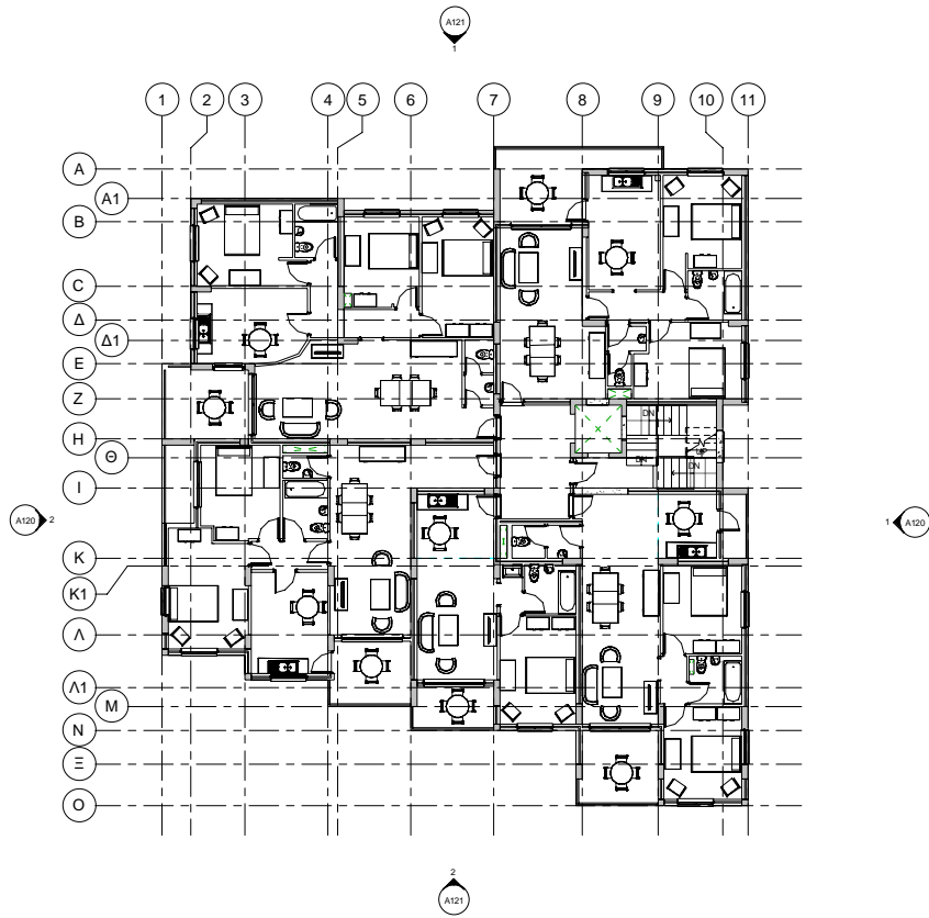
1 1st Floor Plan - Furniture 1 : 100
