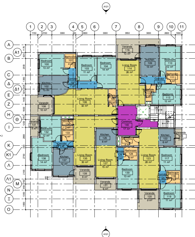
1 1st Floor Plan - Arch 1:100
